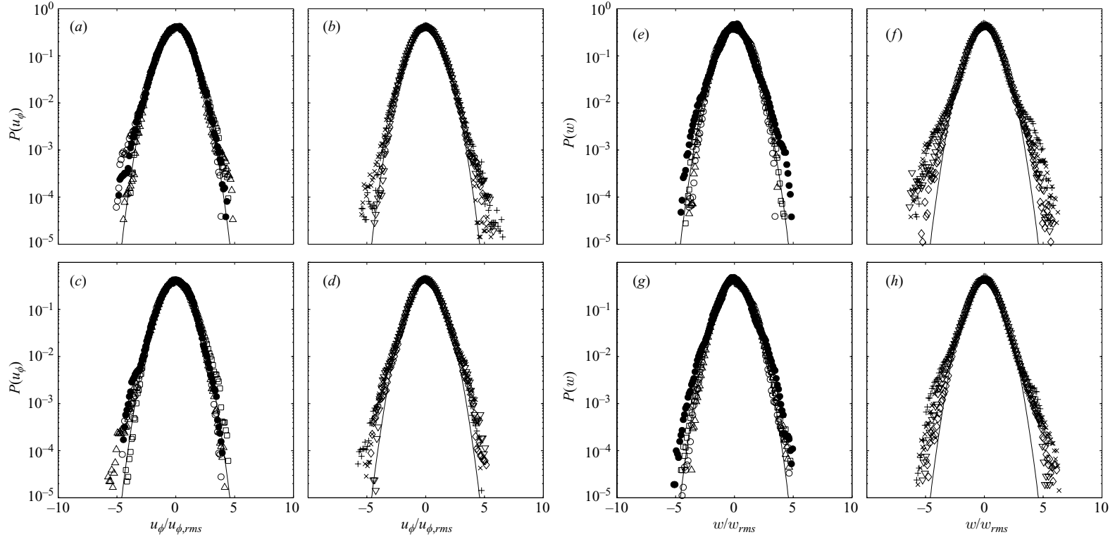
FIGURE 7. Normalized numerical p.d.f.s of horizontal velocity at (a, b) z=0.5H and (c, d) z=0.8H from the simulations; p.d.f.s of vertical velocity at (e, f) z=0.5H and (g, h) z=0.8H . In (a, c, e, g) the Rossby numbers Ro \geq 0.72 are included: Ro = 11.52 (filled circles), 2.88 (open circles), 1.44 (upright triangles) and 0.72 (squares). In (b, d, f, h) the Rossby numbers Ro \leq 0.36 are shown: Ro = 0.36 (diamonds), 0.18 (downward-facing triangles), 0.090 (crosses) and 0.045 (pluses). The solid lines are reference Gaussian distributions.
