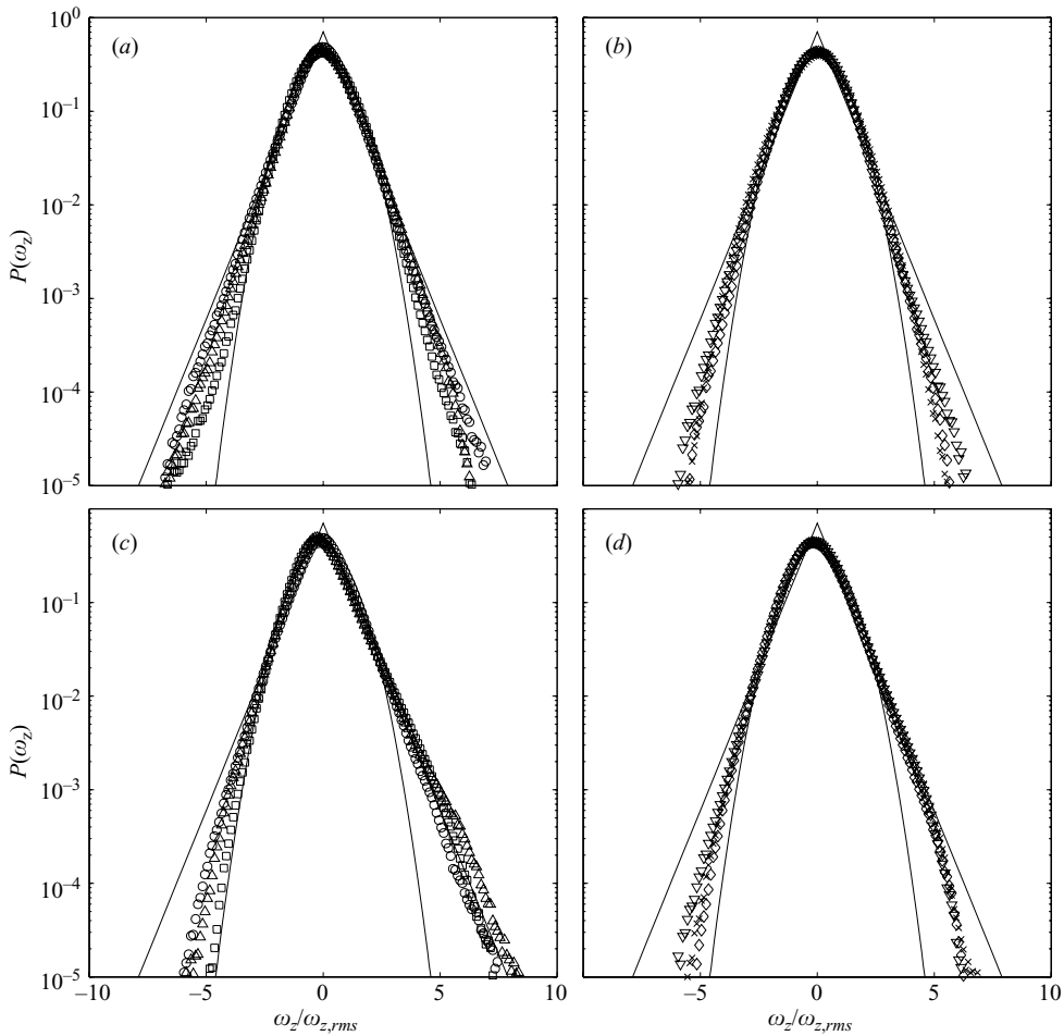
FIGURE 10. Normalized experimental p.d.f.s of vertical vorticity fluctuations \omega_z at (a, b) z = 0.5H and (c, d) z = 0.8H . Reference Gaussian and exponential distributions are also included (solid lines). In plots on the left the Rossby numbers Ro \geq 0.72 are considered: Ro = 2.89 (circles), 1.44 (upright triangles) and 0.72 (squares). On the right the Rossby numbers Ro \leq 0.36 are included: Ro = 0.36 (diamonds), 0.18 (downward-facing triangles) and 0.090 (crosses).
